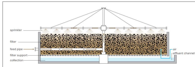
Figure 22: Tricking Filter (Taken from: Tilley, et. al., 2008)
